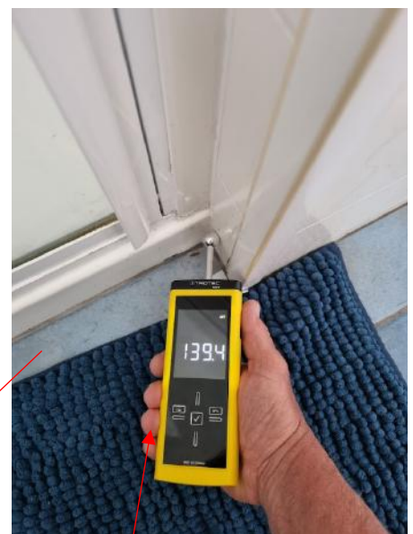
Moisture meter readings are higher than 80, this indicates there is wet materials and is at risk. Further investigation is required
